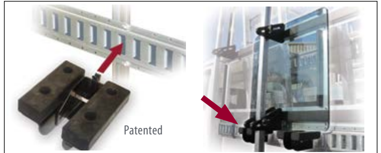
Second Ledge System: transport glass on upper portion of rack when bottom ledge is occupied E-track required (sold separately)
